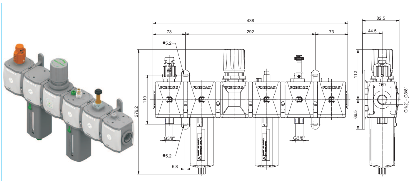
Example : GT173BVKSGB9 : size 3 combined group comprising Shut-off valve, Filter, Regulator, Lubricator, Electrical shut-off valve and Progressive start-up valve Technopolymer threads, G1/2\"
