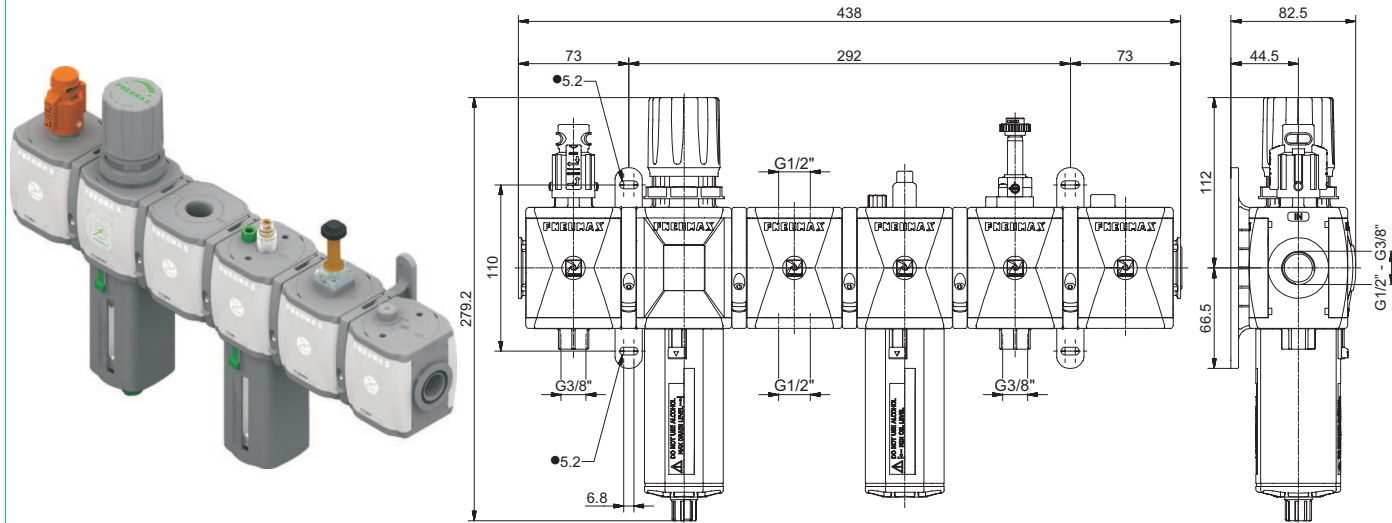
Example : GT173BVNSGB9 : size 3 combined group comprising Shut-off valve, Filter-regulator, Air intake, Lubricator, Electrical shut-off valve and Progressive start-up valve Technopolymer threads, G1/2" connections 0 to 8 bar adjusting range, 20 µm filter pore size and 24V DC(2W) coil
