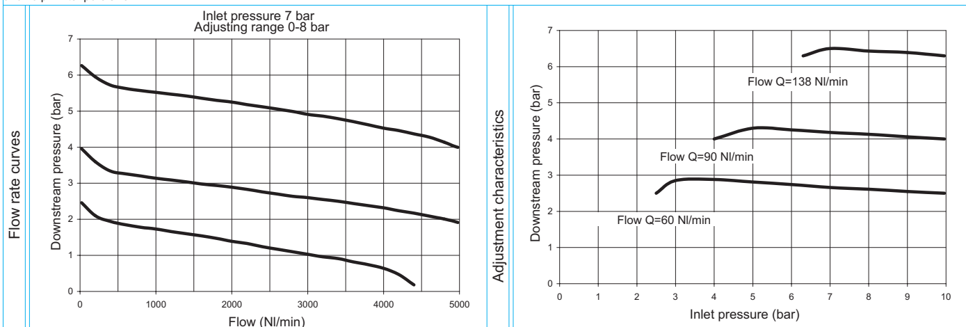
Example : GT173BRG : size 3 combined group comprising Filter-Regulator, Pressure switch and Lubricator Technopolymer threads, G1/2" connections 0 to 8 bar adjusting range and 20 µm filter pore size
