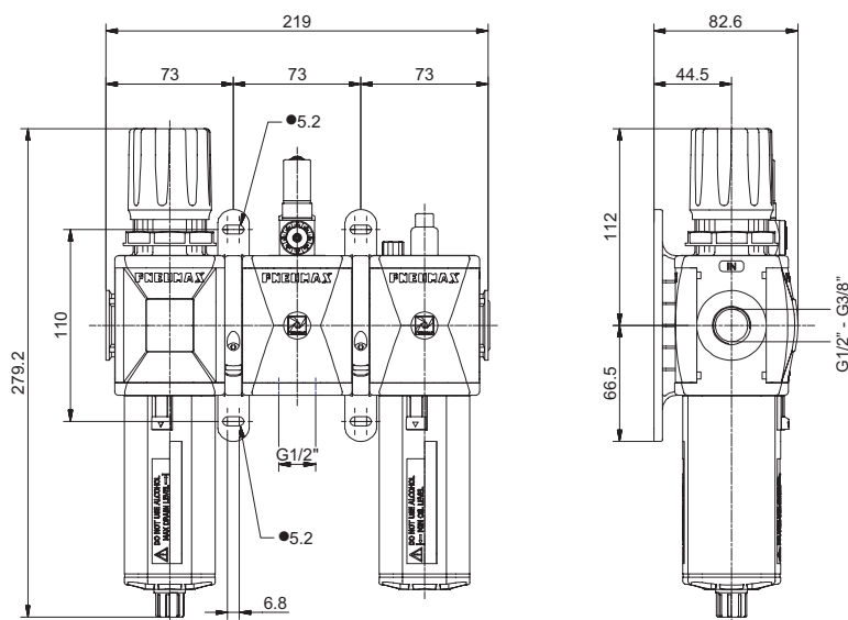
Example : GT173BRG : size 3 combined group comprising Filter-Regulator, Pressure switch and Lubricator Technopolymer threads, G1/2" connections 0 to 8 bar adjusting range and 20 µm filter pore size
