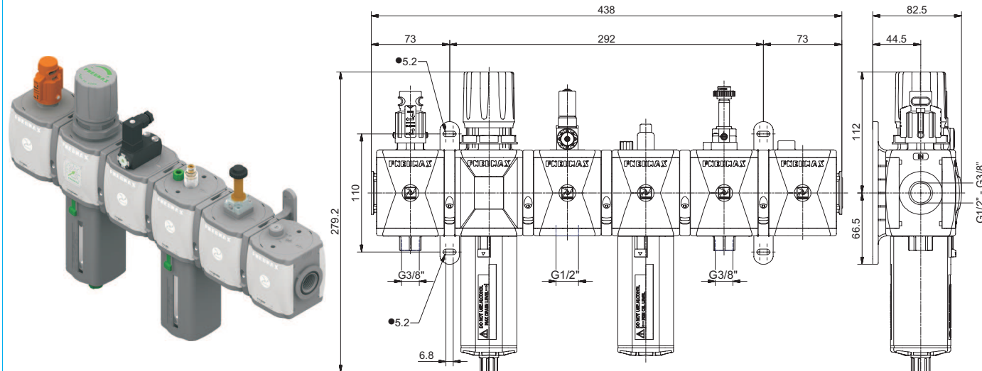
Example : GT173BVRSSB9 : size 3 combined group comprising Shut-off valve, Filter-regulator, Pressure switch, Lubricator, Electrical shut-off valve and Progressive start-up valve Technopolymer threads, G1/2\" connections 0 to 8 bar adjusting range, 20 \mu m filter pore size and 24V DC(2W) coil
