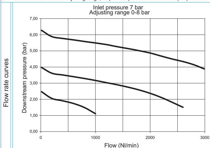
Example : GT173BVNSGB9 : size 3 combined group comprising Shut-off valve, Filter-regulator, Air intake, Lubricator, Electrical shut-off valve and Progressive start-up valve Technopolymer threads, G1/2" connections 0 to 8 bar adjusting range, 20 µm filter pore size and 24V DC(2W) coil
