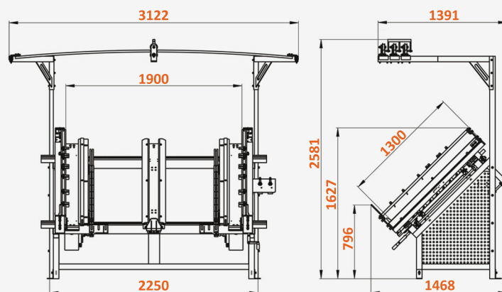
The size of Pneumatico PT-1900 table in mm
